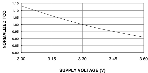
NORMALIZED T_{CO} VS. V_{CC}
